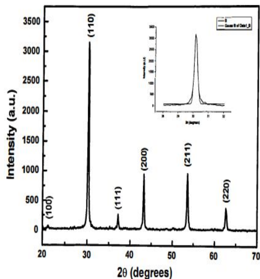
Figure 1: The XRD pattern of as-prepared BaZrO_3 nanocrystals. A close-up view of (110) predominant peak in the inset is used to calculate the grain size of the powder
