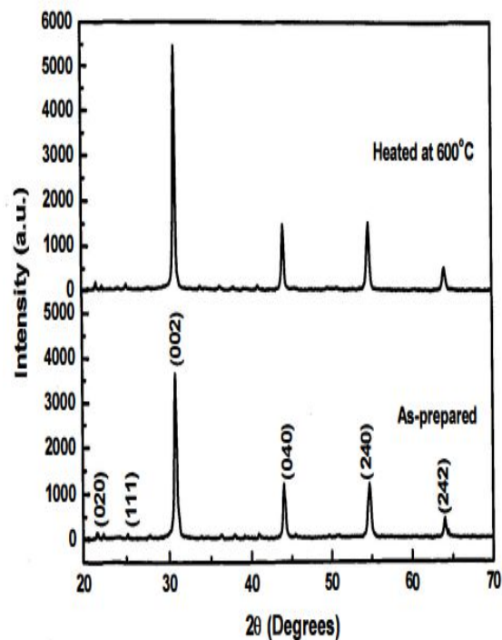
Figure 2: The XRD pattern of as-prepared and annealed SrZrO 3 nanocrystals at 600 °C.
